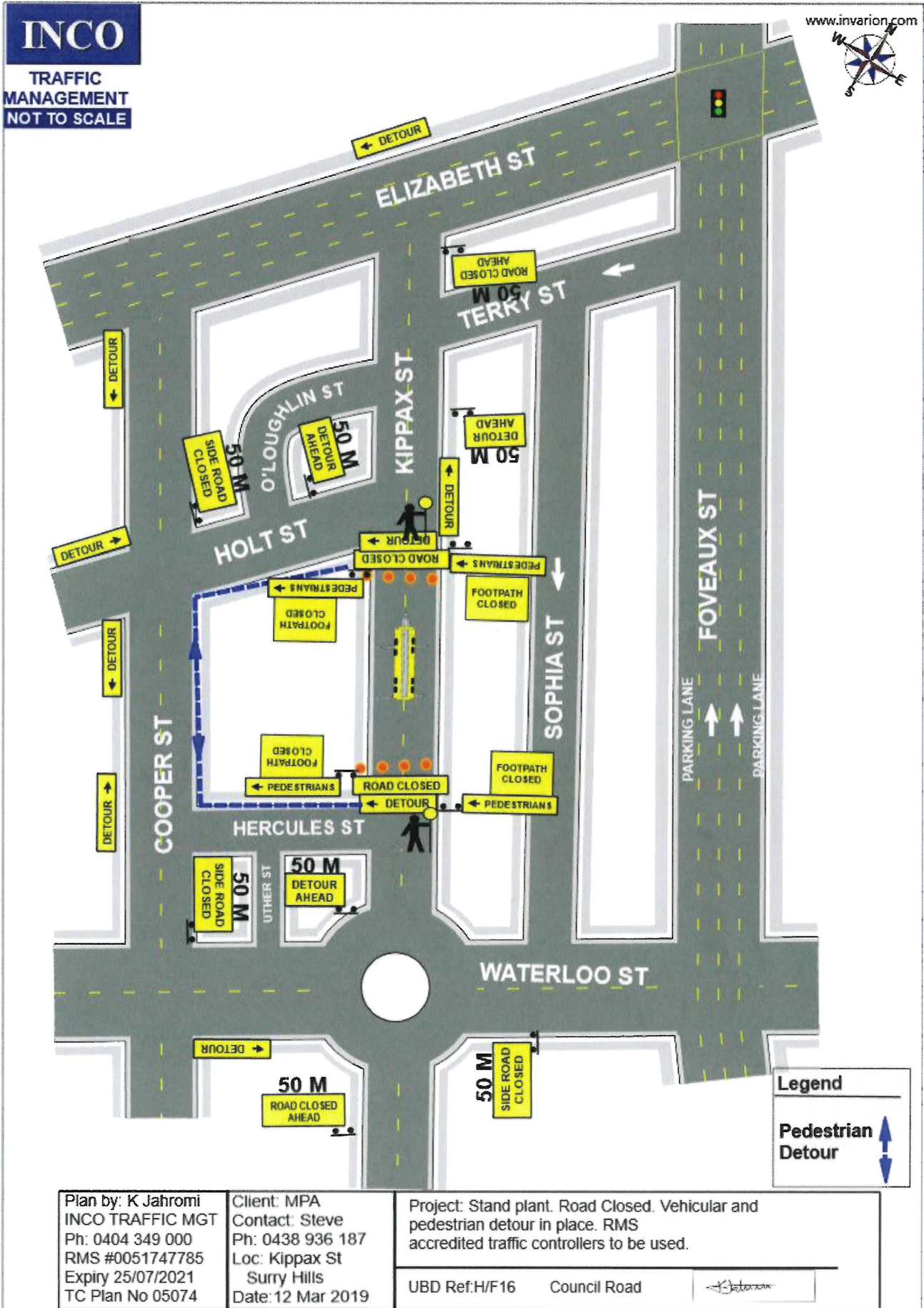
FIGURE 4: TRAFFIC CONTROL PLAN
