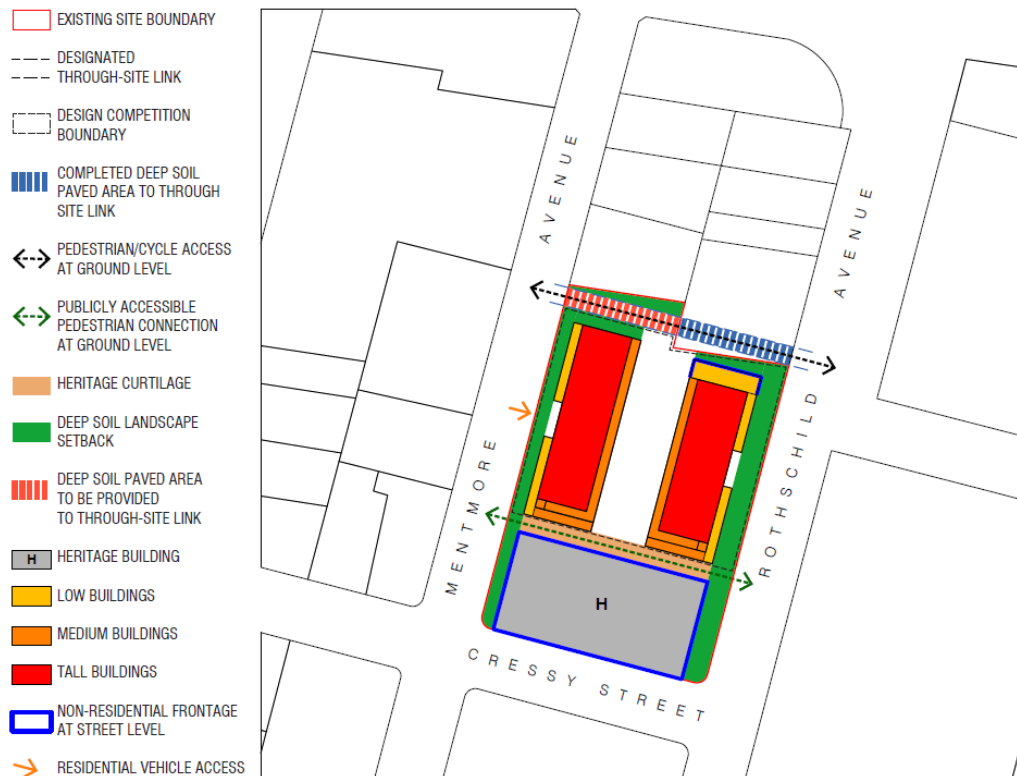
Figure 6.XX: Structure and land use plan
