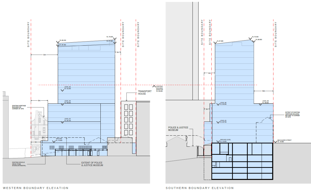
Figure 23: Proposed maximum envelope elevations to the western boundary (left) southern boundary (right)
