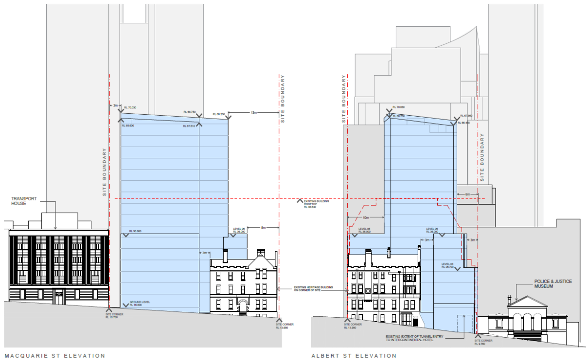
Figure 22: Proposed maximum envelope elevations to Macquarie Street (left) and Albert Street (right)
