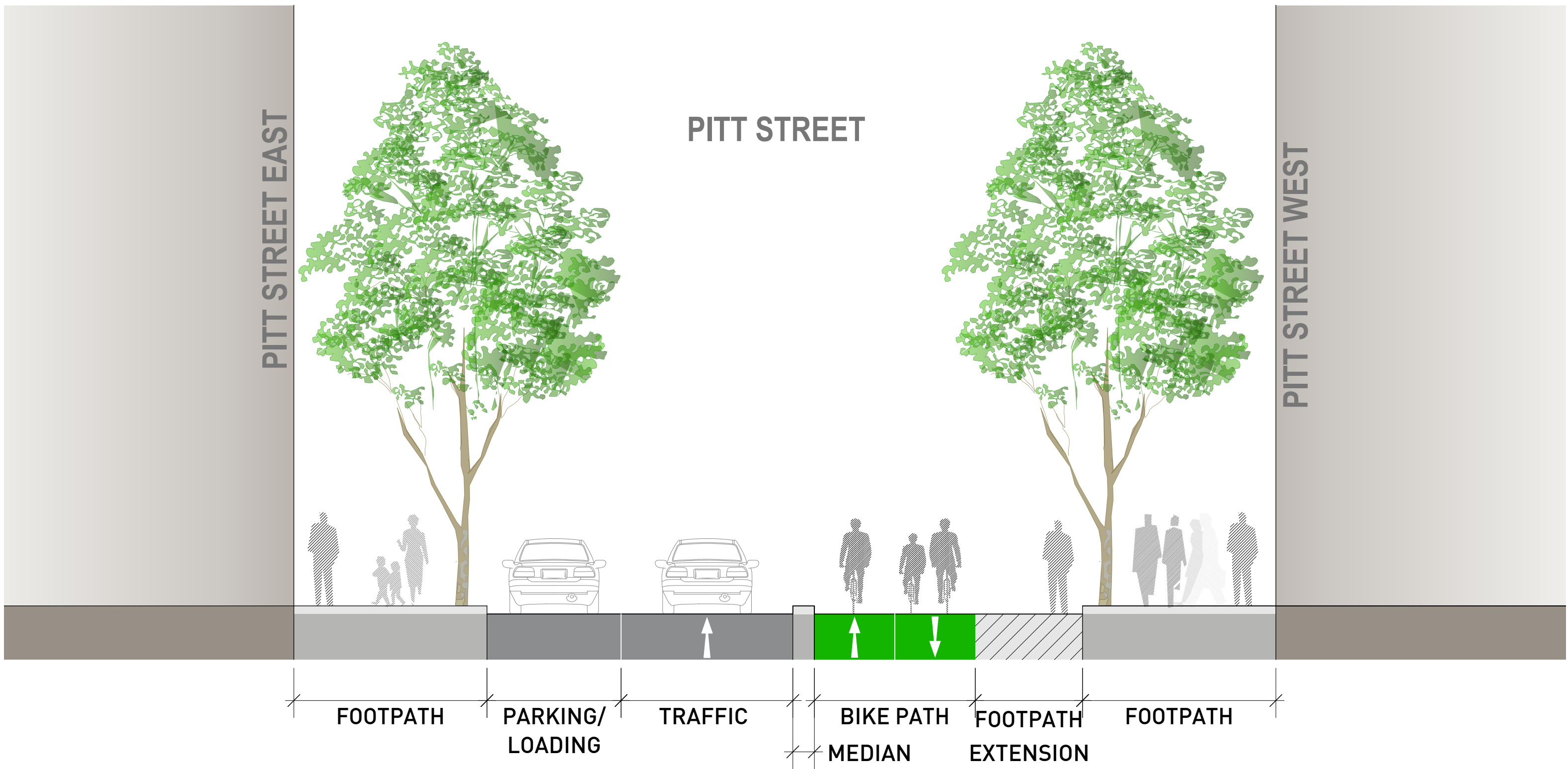
Typical Street Cross Section A-A
