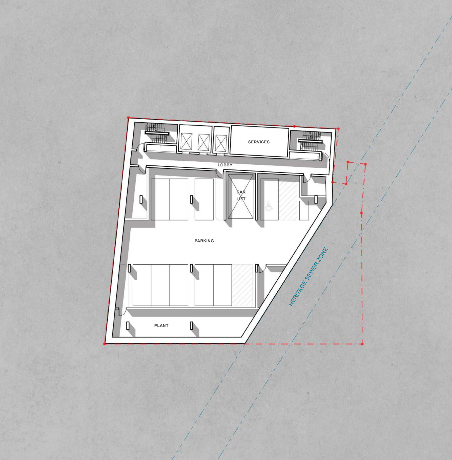
BASEMENT 3-4 PLAN
