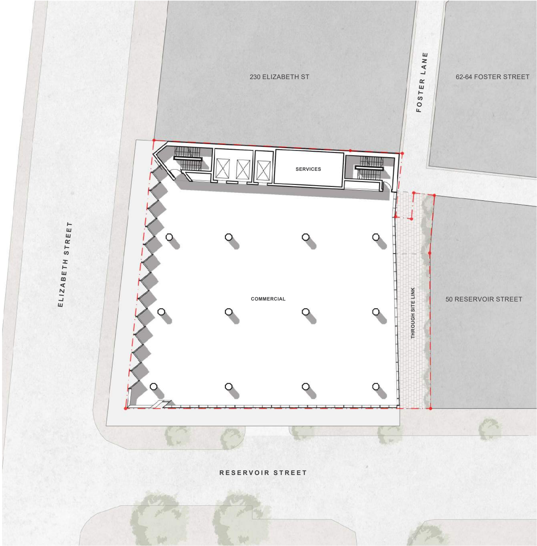
TYPICAL FLOOR PLAN - L1 TO L7 COMMERCIAL GFA 714 m 2
