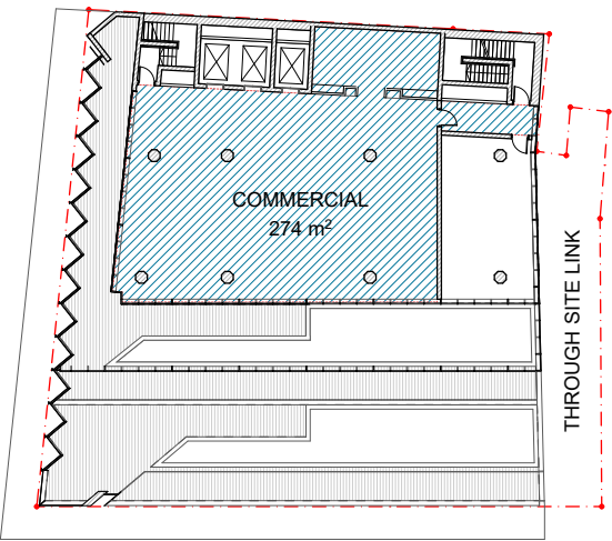
LEVEL 9 PLAN
