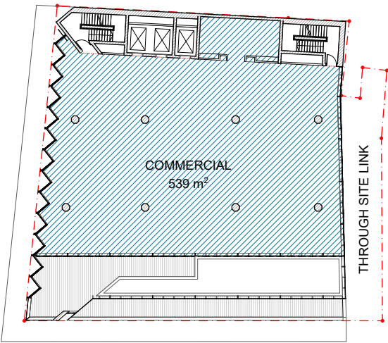
LEVEL 8 PLAN
