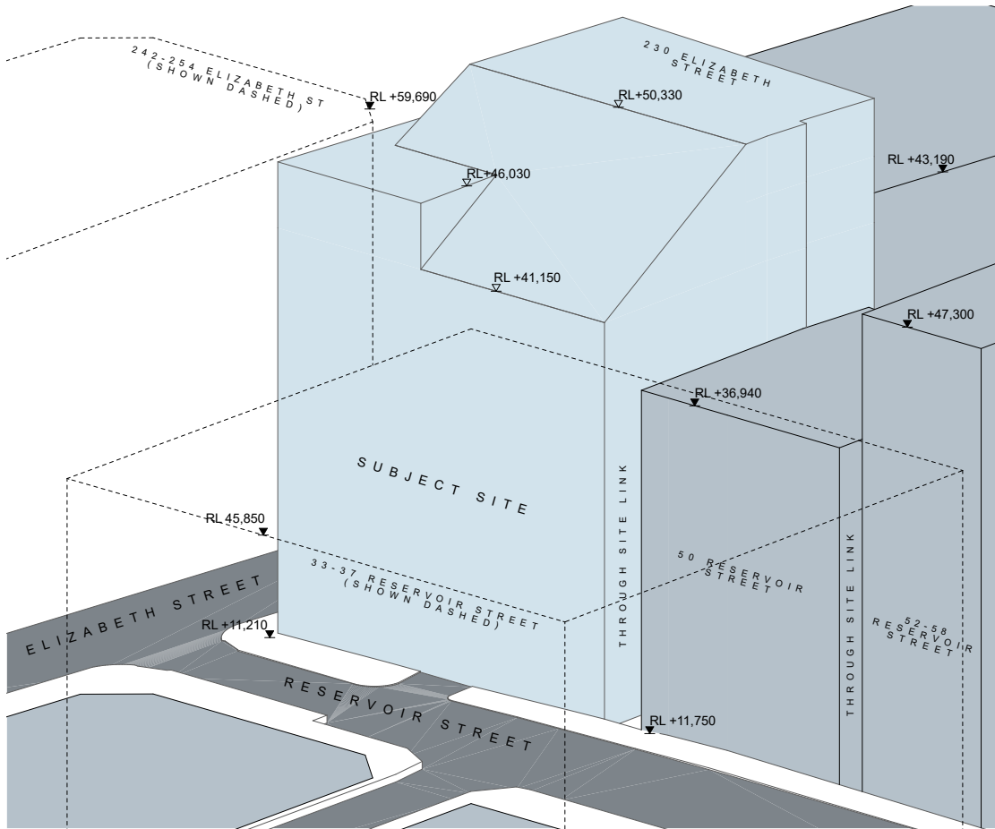
ISOMETRIC - PROPOSED ENVELOPE
