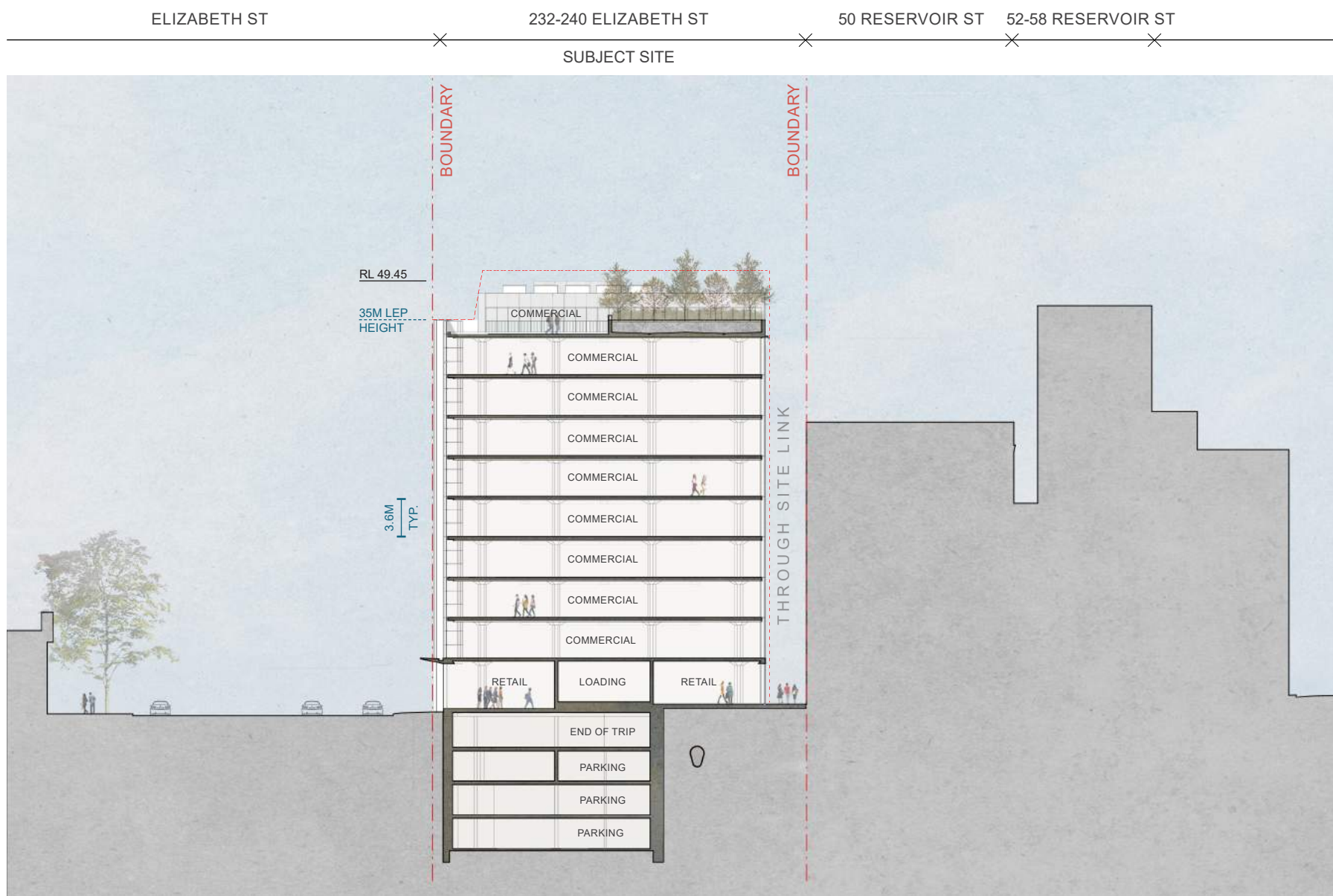
SECTION BB
