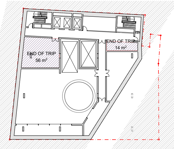
BASEMENT 1 PLAN
